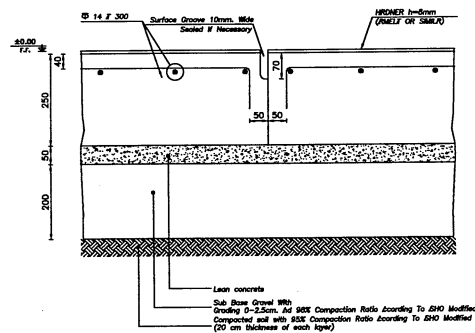
CONTRACTION JOINTS
