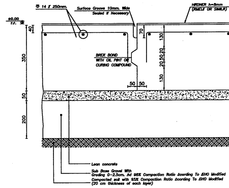
CONSTRUCTION JOINTS
