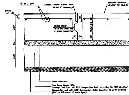
CONSTRUCTION JOINTS
