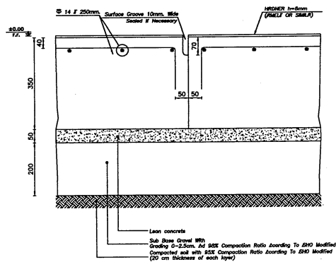
CONTRACTION JOINTS
