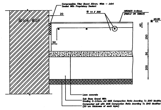
ISOLATION JOINT AGAINST THE WALLS
