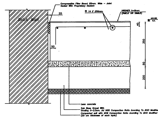
ISOLATION JOINT AGAINST THE WALLS
