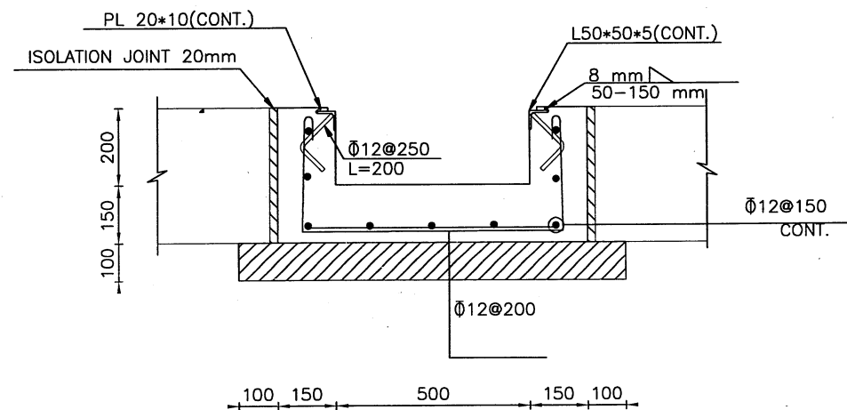
SECTION E-E Scale=1:10
